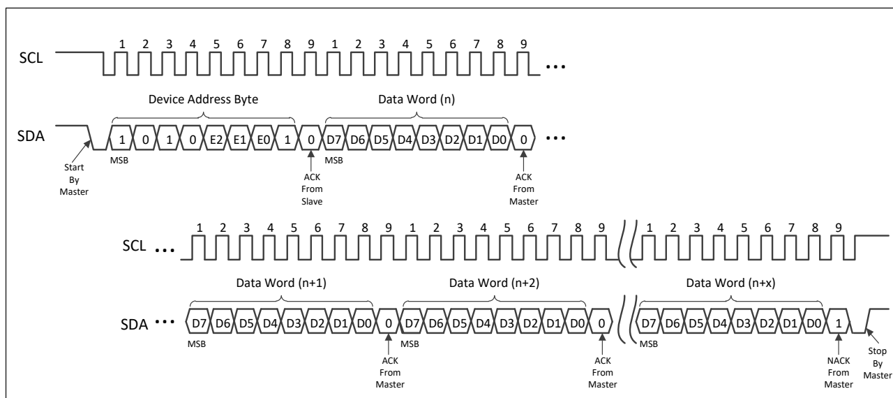
Figure 5–12 Sequential Read
