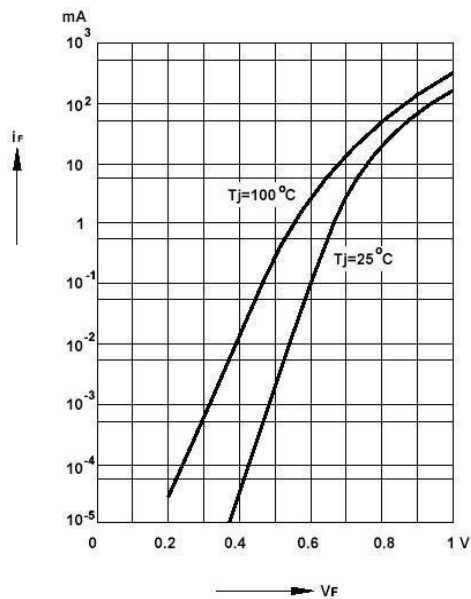
Forward characteristics
