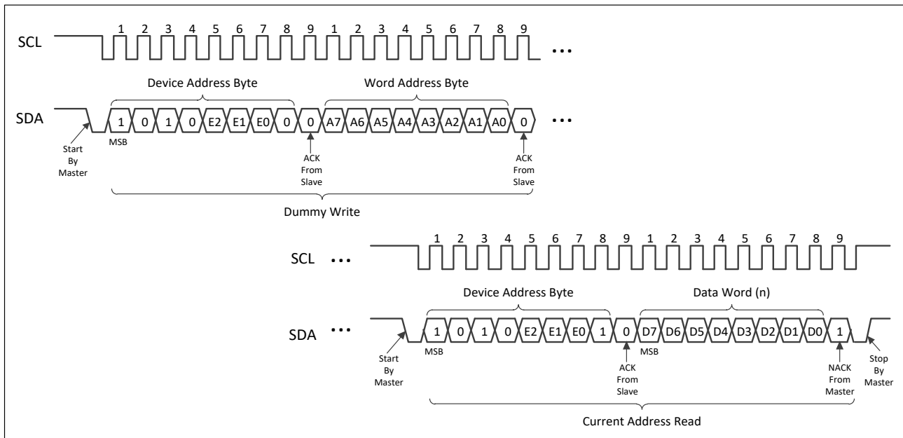
Figure 5-11 Random Read
