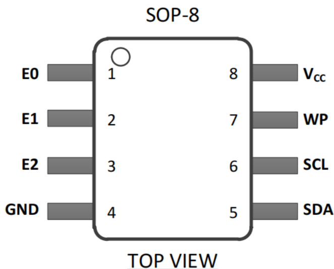
Figure 1-1 Pin Configuration
