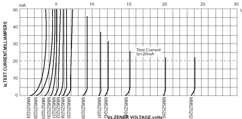
Breakdown characteristics
