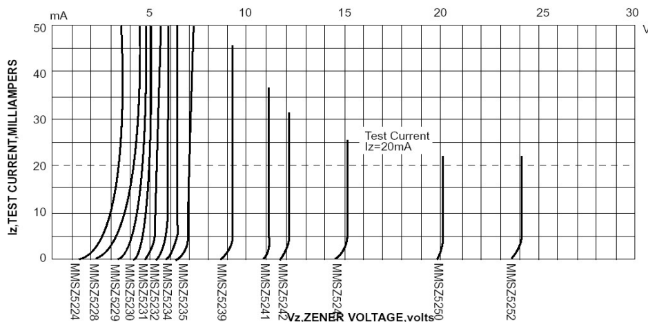
Breakdown characteristics
