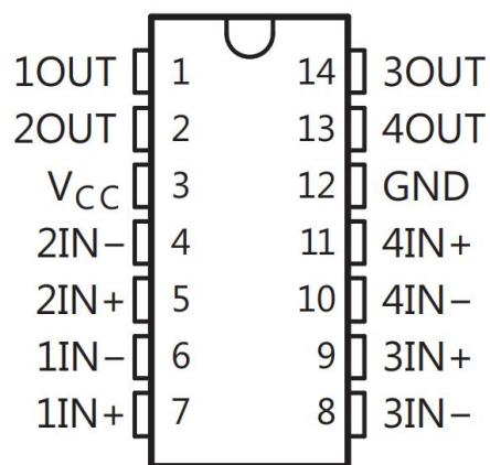
SOP14
