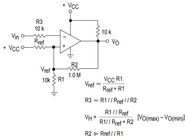
Figure 1. Inverting Comparator with Hysteresis
