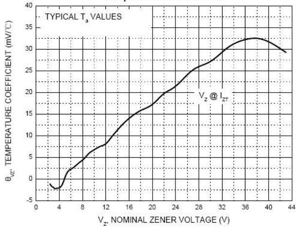
Temperature Coefficients
