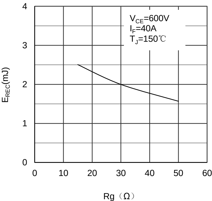
Figure 10. Switching Energy vs Gate Resistor Diode
