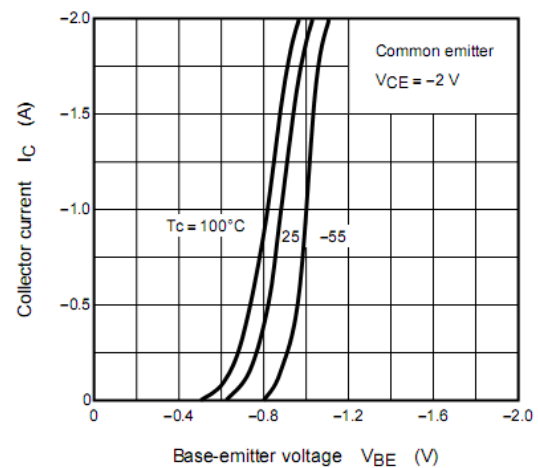
Figure 4. Base-Emitter Saturation Voltage
