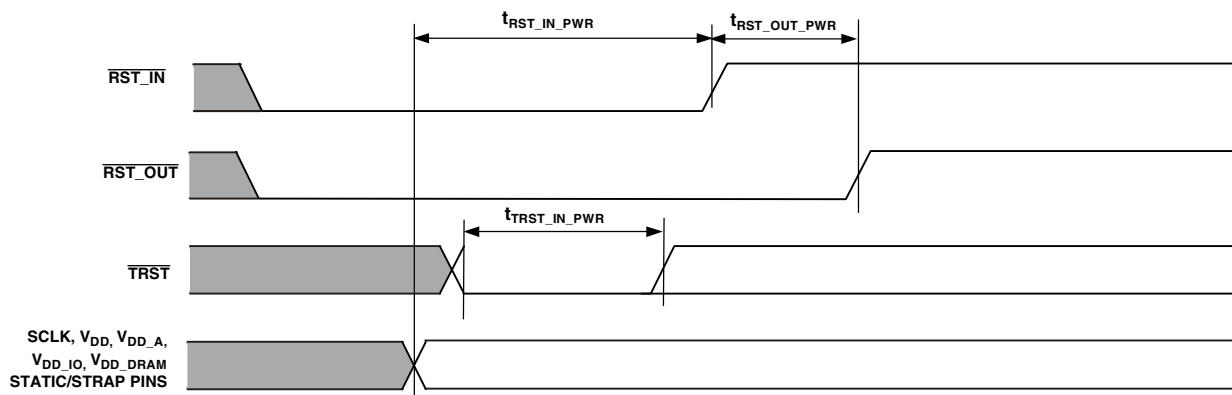
Figure 13. Power-Up Reset Timing
