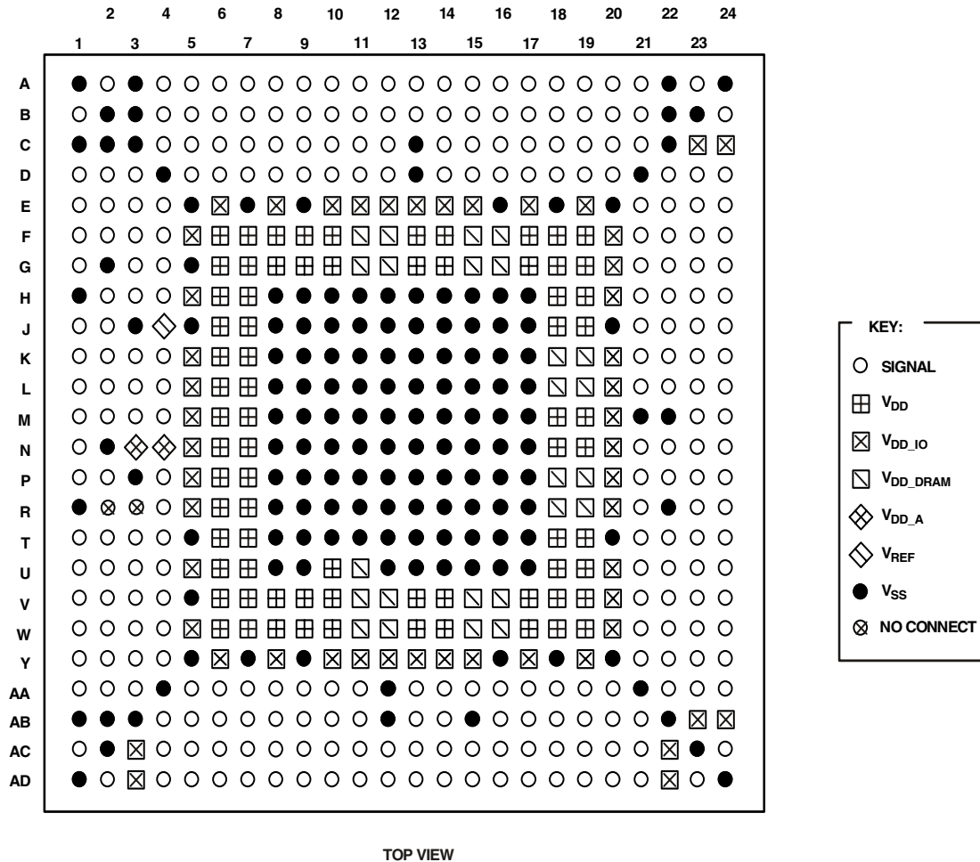
Figure 46. 576-Ball BGA_ED Pin Configurations (Top View, Summary)
